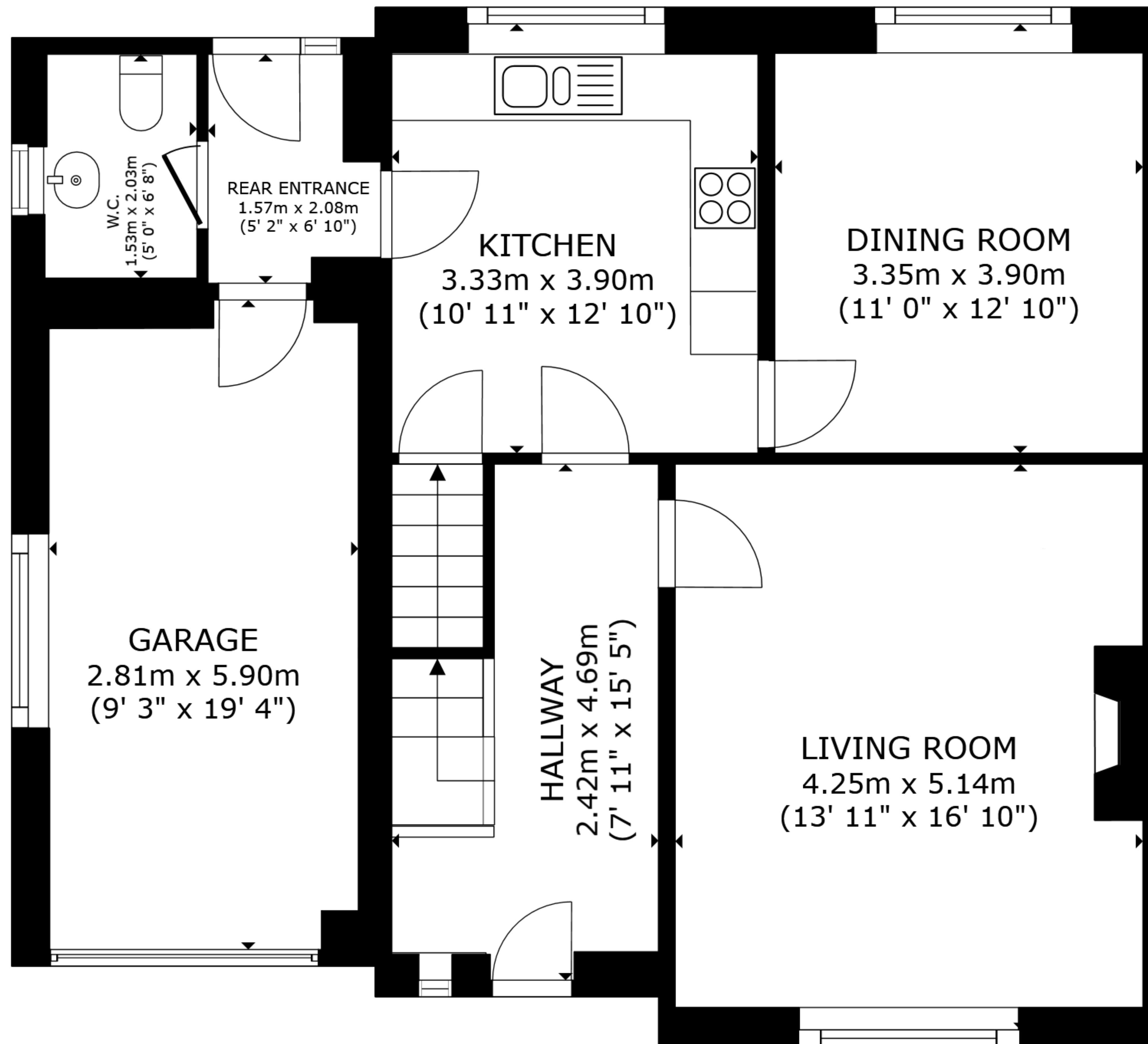
FLOOR 1
