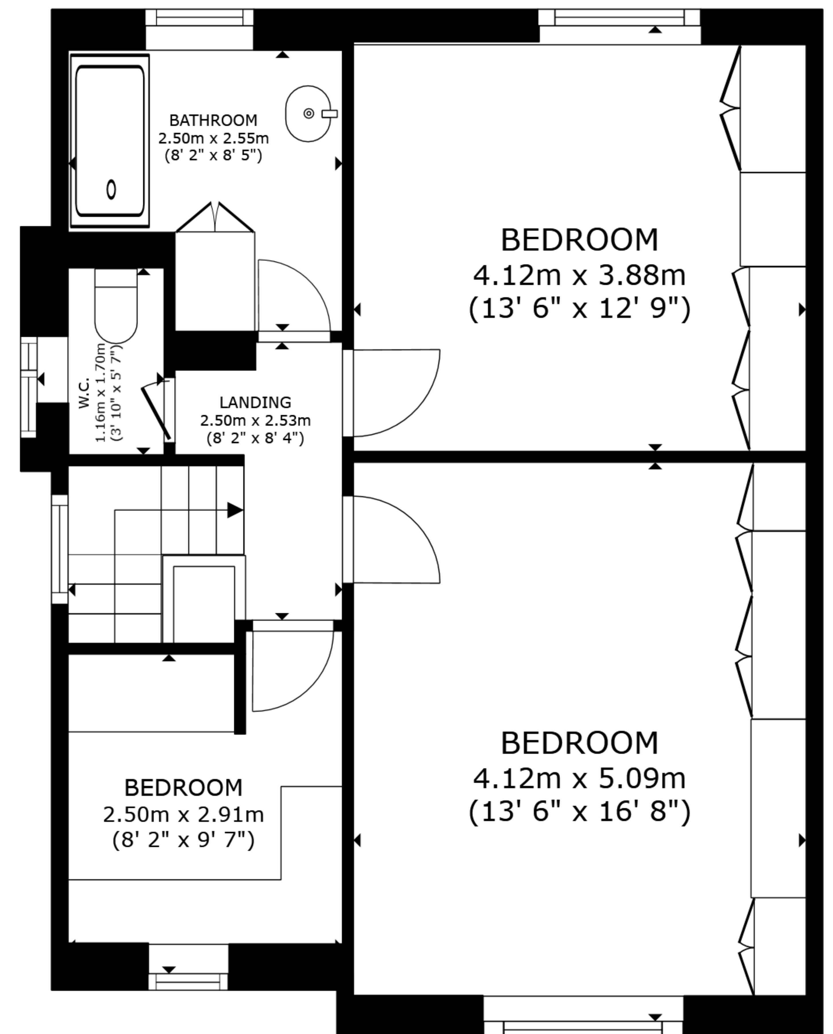
FLOOR 2
